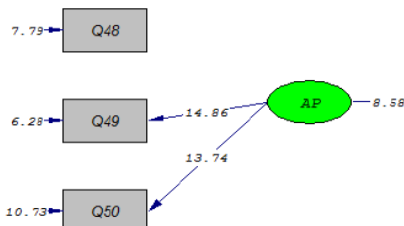
Chi-Square=1.18, df=1, P-value=0.27769, RMSEA=0.029
