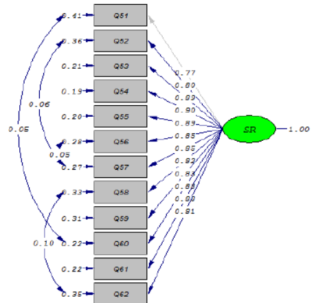
Chi-Square=73.29, df=37, P-value=0.00035, RMSEA=0.052
